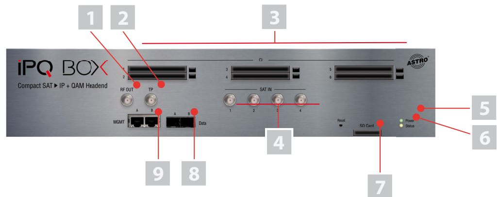
Figure 1: IPQ BOX pin assignment
