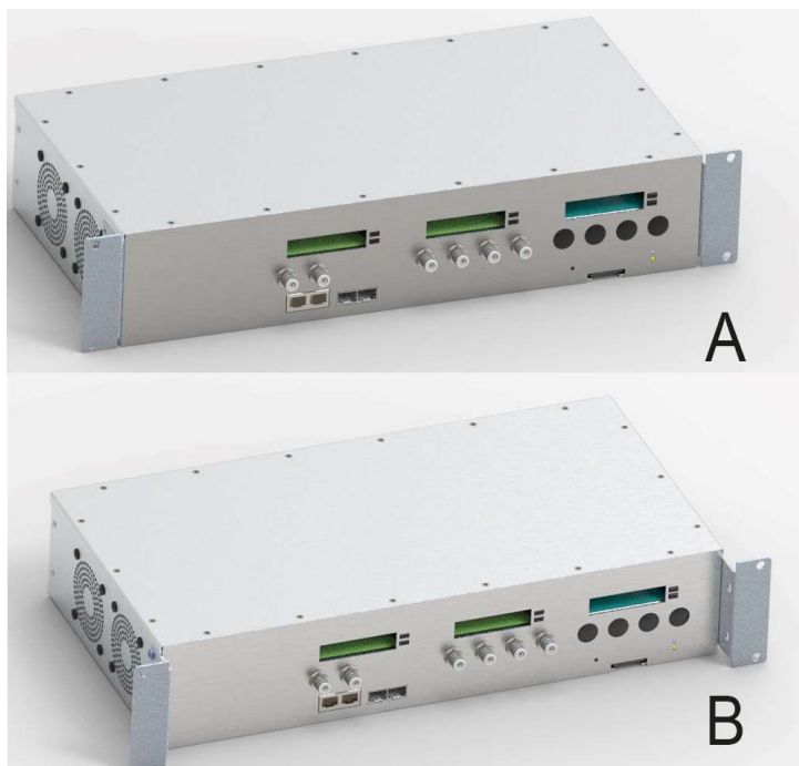
Figure 3: Mounting in a 19 inch cabinet
