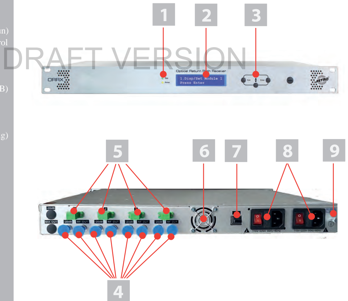
Figure 1: ORRX front and rear side
