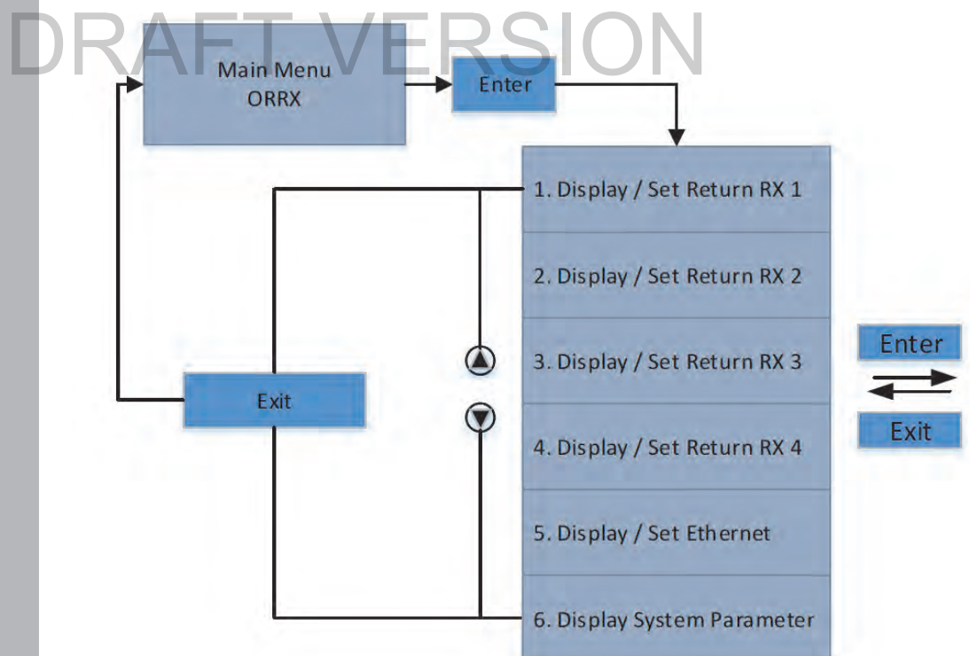
Figure 4: LCD panel menus
